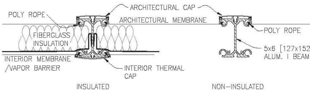
5"x6" BEAM SECTION 1 1/2"=1'-0"
