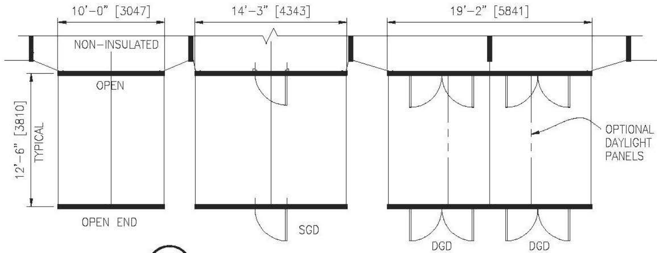
PLAN VIEW 1/8"=1'-0"
