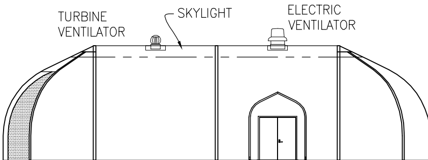
ELEVATION 1/16"=1'-0"
