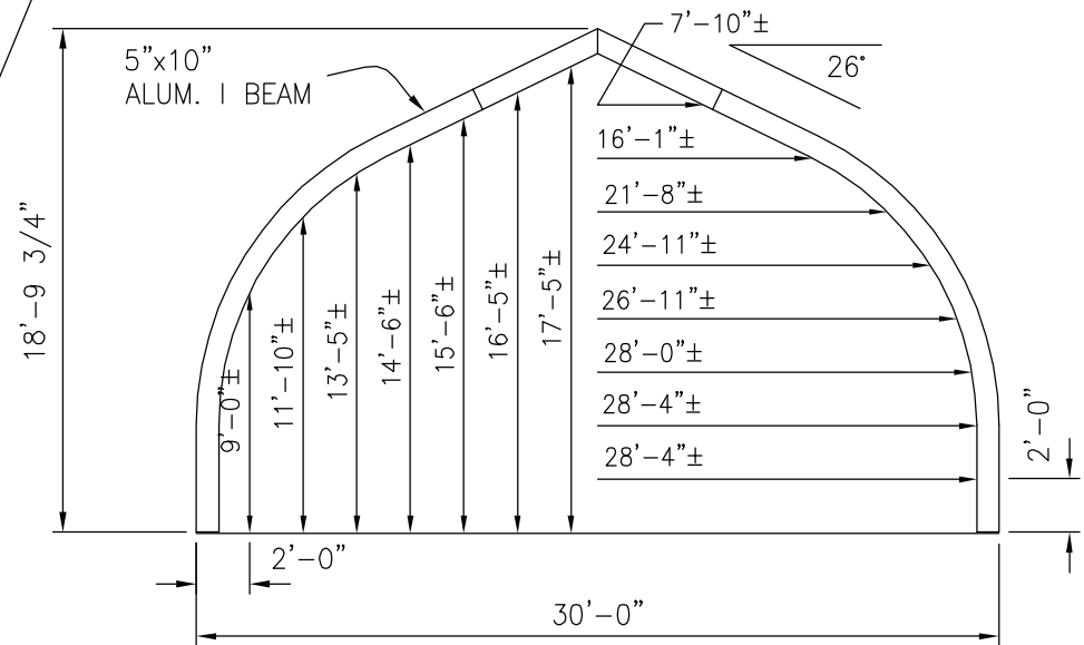
SECTION 30'-0" STRUCTURE 1/8"=1'-0"
